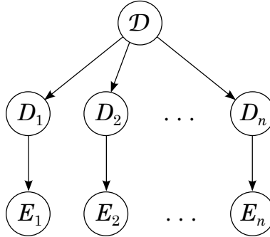
Figure 1: Bayes net for modeling successful instances of creative abduction
