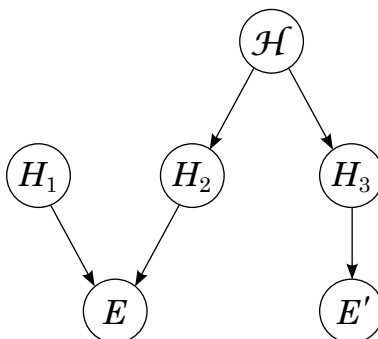
Figure 3: Bayes net modeling Laudan and Leplin’s (1991) solution to the problem of underdetermination
